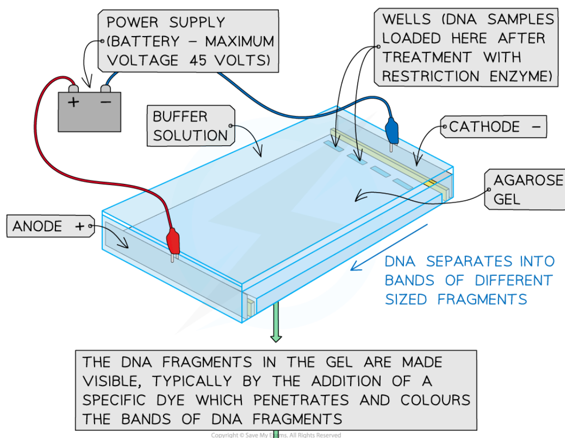
Gel electrophoresis diagram
