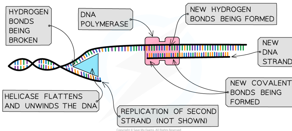
Function of helicase and DNA polymerase diagram
